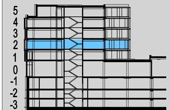
CROSS SECTION
